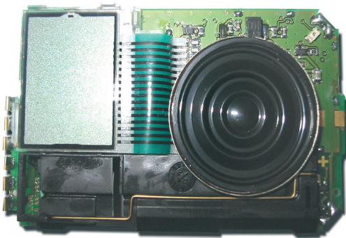
LC-Display / Loudspeaker
