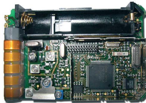
Antenna / Crystal
